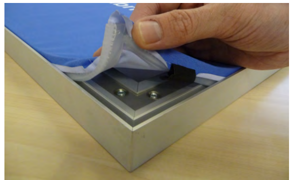
SINGLE SIDED WALL MOUNT
